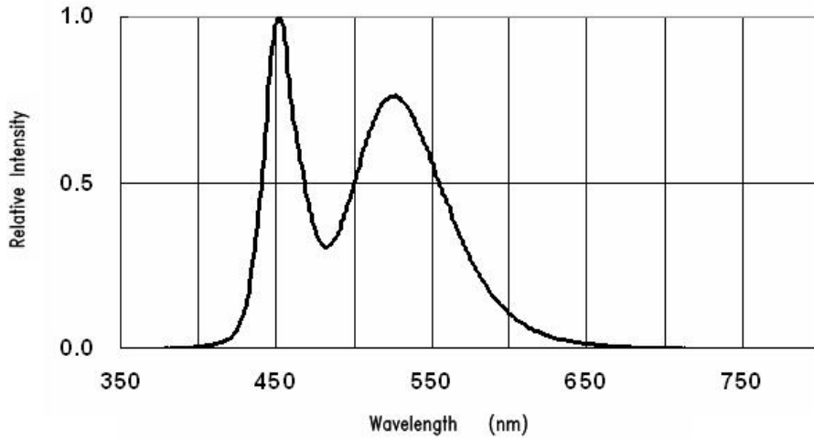
Fig.1 RELATIVE INTENSITY VS. WAVELENGTH
